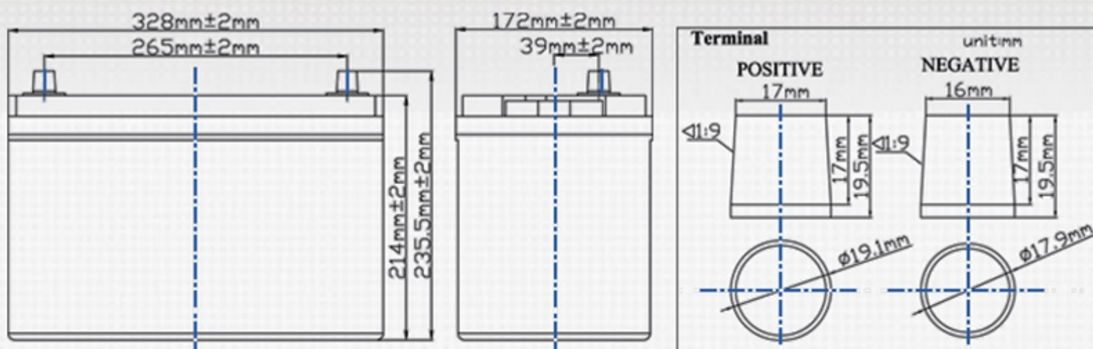
DETAIL A
