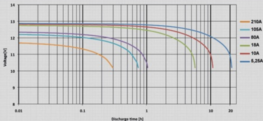
Discharge Curves
